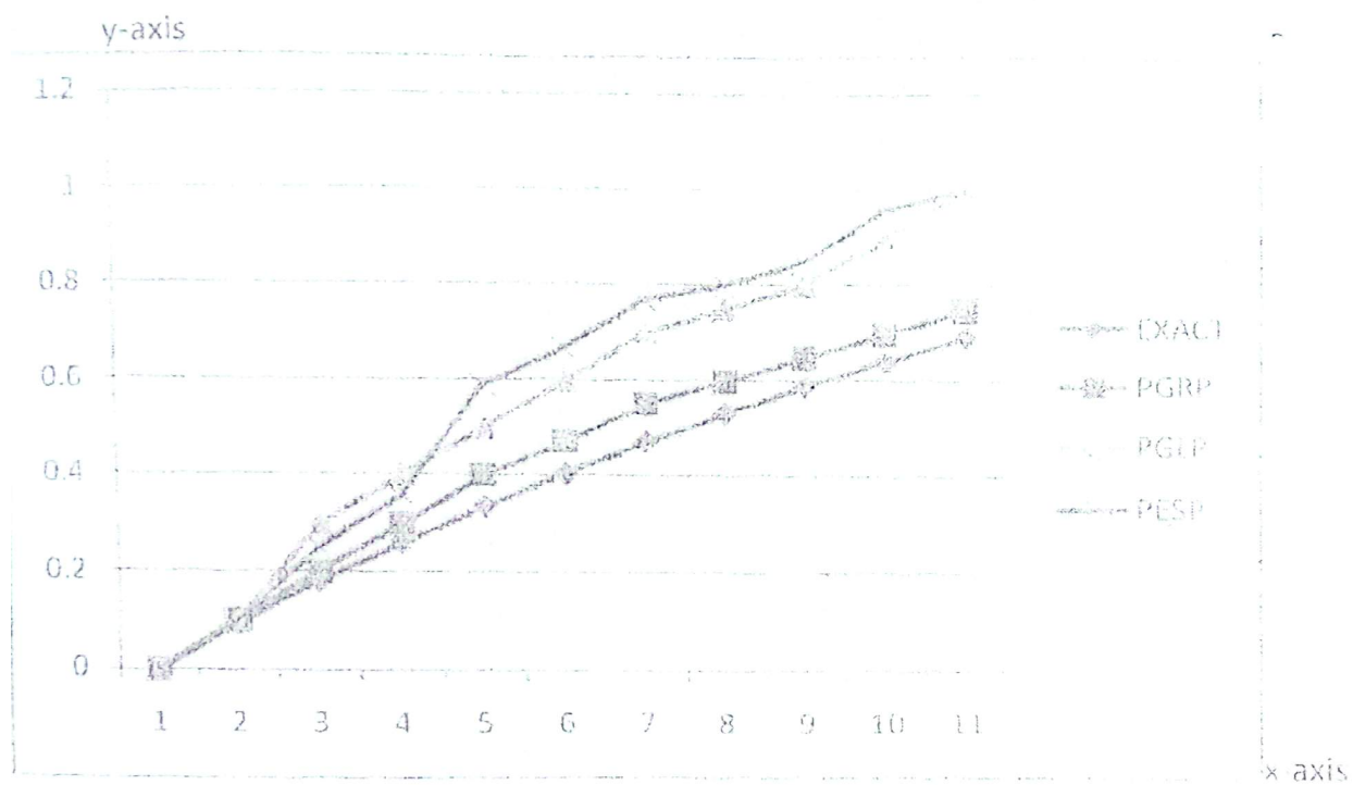
Figure 3: Graphical representation of example 3 for the exact solution and the collocation method.
