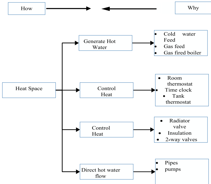
Figure 5: A Function Logic Diagram of BS Heat Installation
