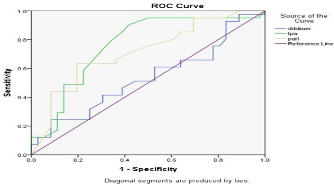
Fig.1: Receiver' Operation Characteristic curve for determining the Sensitivity of tPA, PAI-1 and D-dimer as markers of severity of Pre-eclampsia in the laboratory
