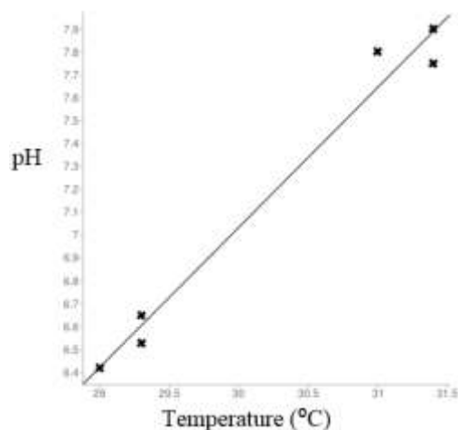
Figure I: Correlation coefficient scatter plot for the temperature and pH of water samples from Ilorin, Nigeria
